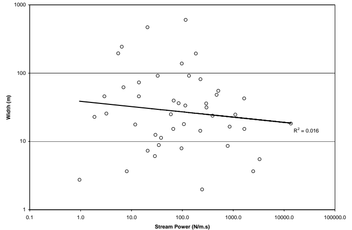
FIGURE 2. The Relationship of Width Versus Stream Power for a Variety of River Sizes at High Flows. Data from Barnes, 1967; Hicks and Mason, 1991; Annable, 1994; and Williams and Rosgen, 1989. From Rosgen (2006c; reprinted with permission of ASCE).
