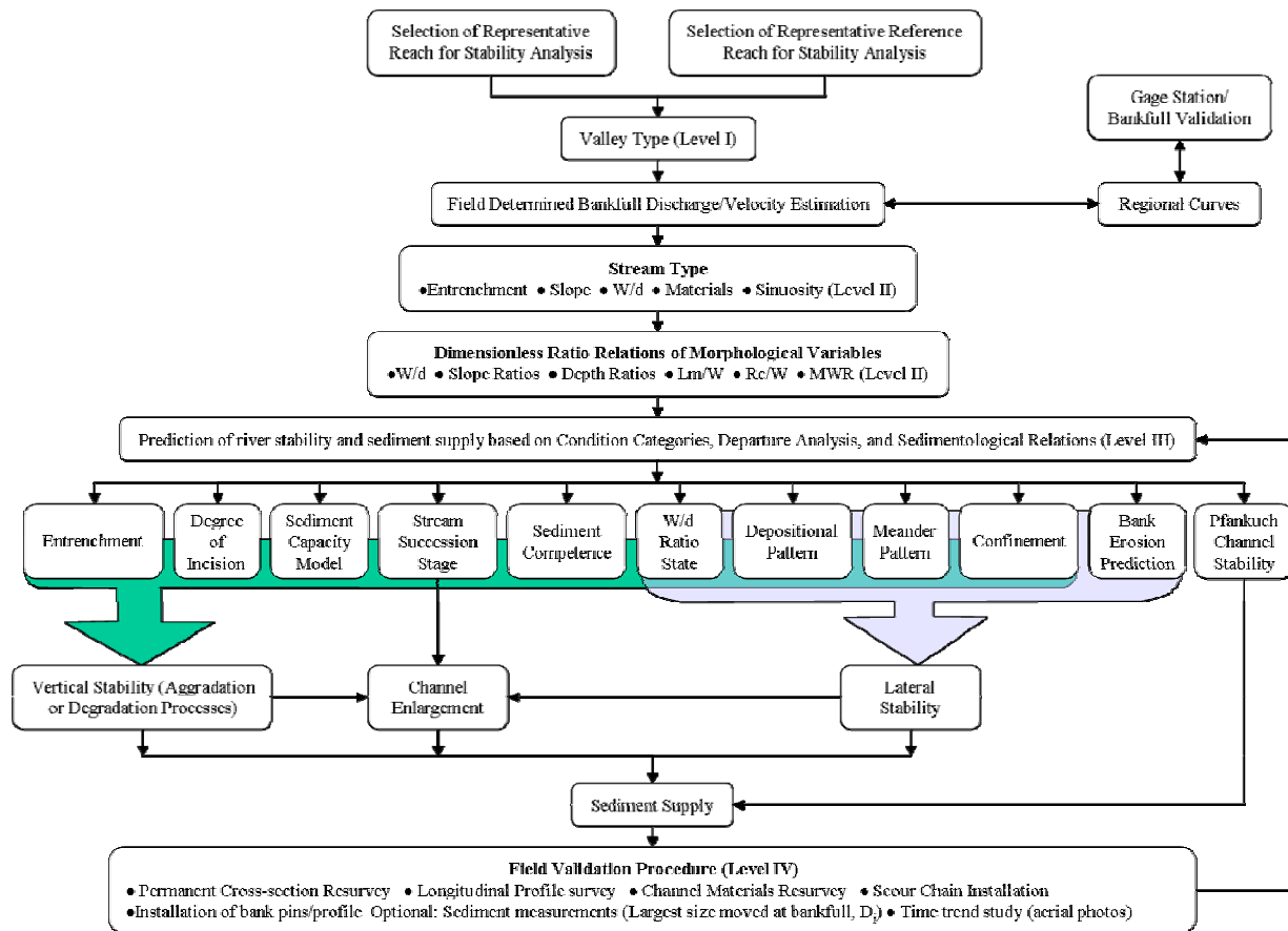
FIGURE 1. Generalized Flowchart of Application of the Four Assessment Levels of Channel Morphology, Stability Ratings, and Sediment Supply Used in Natural Channel Design (In Rosgen, 2004, 2006b, c, 2007).
