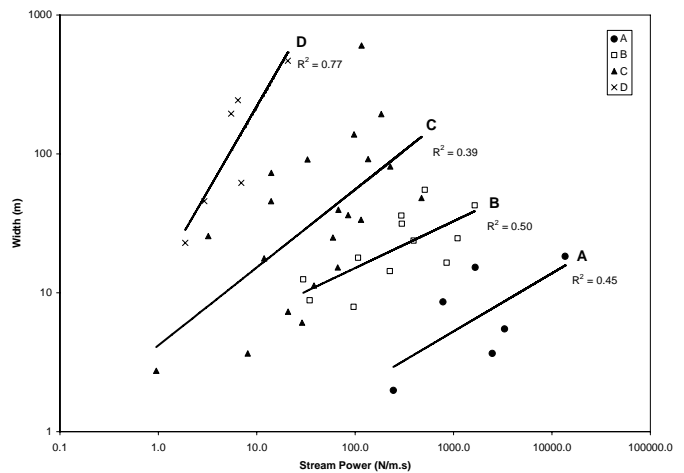
FIGURE 3. A Stratification of the Data in FIGURE 2 by Major Stream Type Showing Relationship of Width Versus Stream Power. From Rosgen (2006c; reprinted with permission from ASCE).
