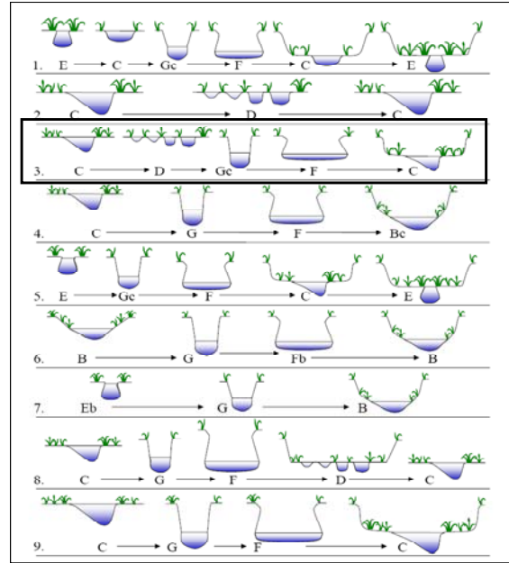
FIGURE 4. Various Successional Stage Scenarios Highlighting Scenario #3 for the Weminuche Creek Example (Rosgen, 2001a, 2003, 2006c, e, 2007; USEPA, 2006).
